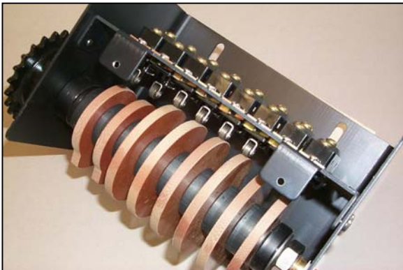
Limit Switch detail
